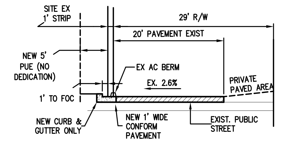
YOSEMITE WAY TYPICAL SECTION
