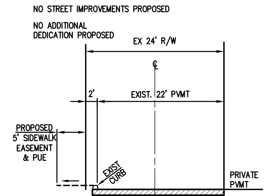
WHEELER AVE TYPICAL SECTION
