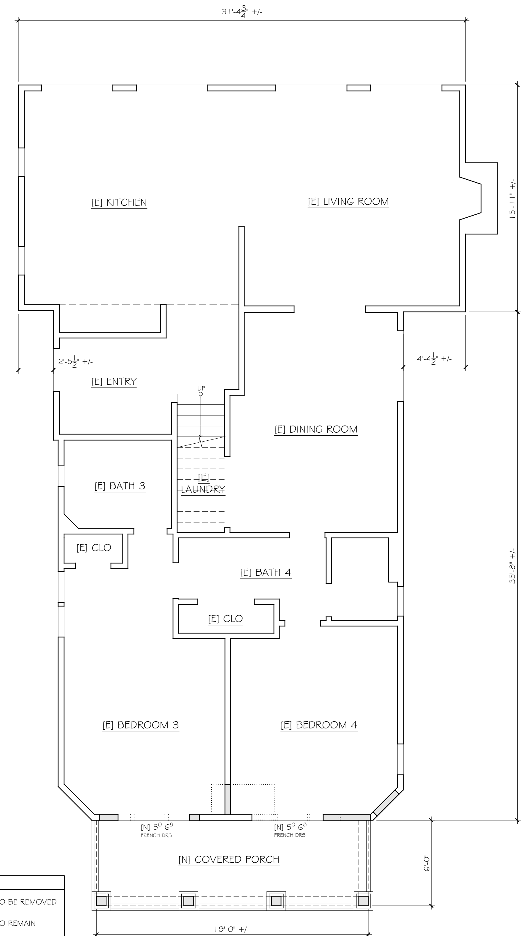
PROPOSED 1ST FLOOR PLAN 1/4" = 1'-0"
