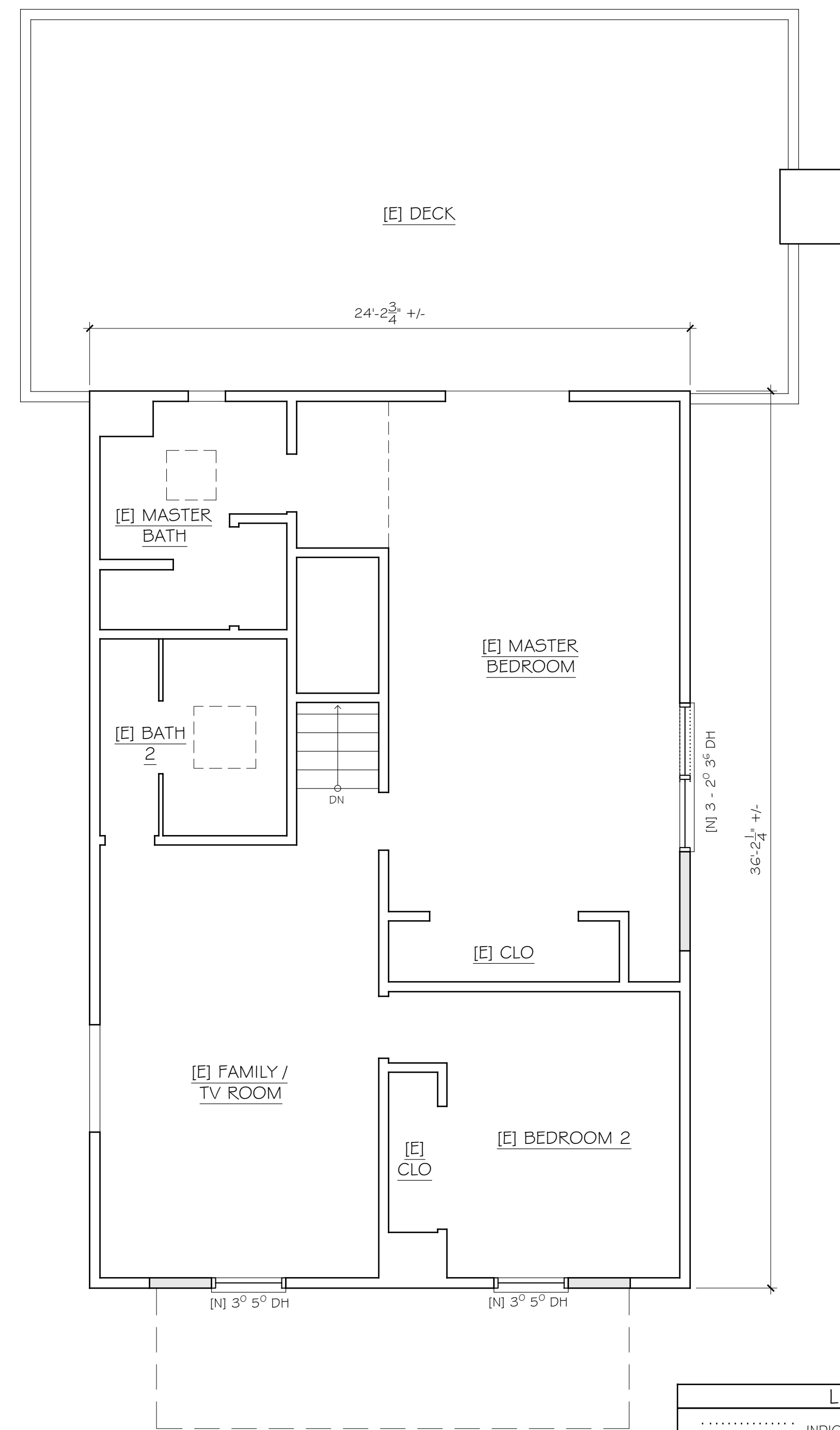
PROPOSED 2ND FLOOR PLAN 1/4" = 1'-0"
