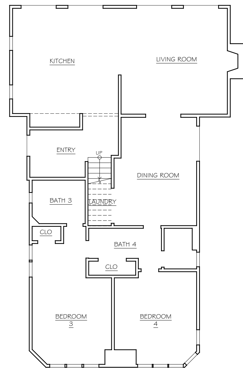
EXISTING 1ST FLOOR PLAN 1/8" = 1'-0"
